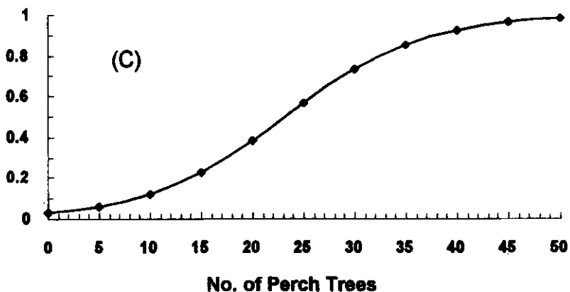
Figure 1. Probability of Madagascar Fish-Eagle use of nest trees, perch trees, and nest sites as a function of nest-tree height (A), perch-tree height (B), and number of shoreline perch trees (C), in the region of Antsalova Madagascar, 1994. Probabilities were calculated by inserting different values of the explanatory variable (tree height or number of perch trees) into the equation resulting from stepwise logistic regression analysis.
